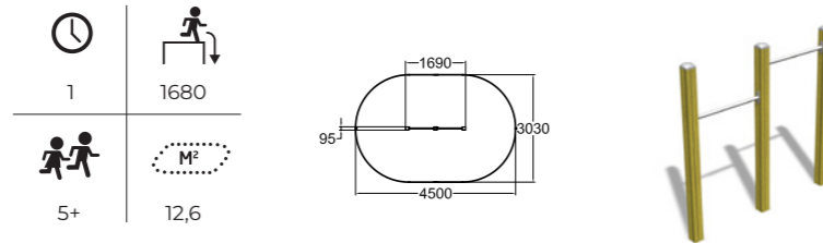
175010 Chinning Bars for 2
