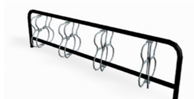
RF7620AM Urban A Double Sided Bicycle Rack L x W x H: 2080 mm x 400 mm x 550 mm Underground concrete foundation.
