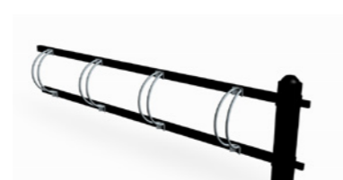
RF9003M Ströget B Bicycle Rack Extension for RF9002M L x W x H: 2000 mm x 220 mm x 600 mm Underground concrete foundation.
