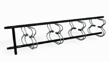
RF7620BM Urban B Bicycle Rack Extension for RF7620AM L x W x H: 2000 mm x 400 mm x 550 mm Underground concrete foundation.
